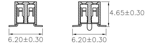
TYPE 1 W/O POST
