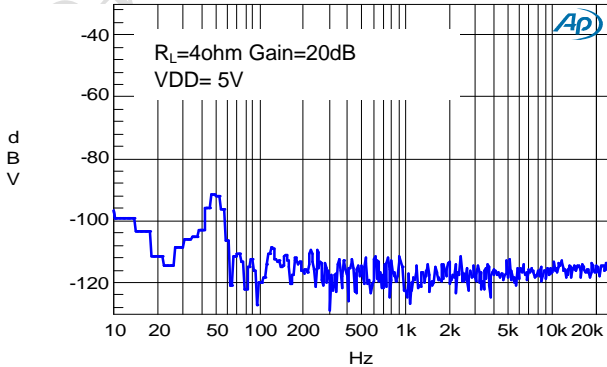
NOISE FLOOR FFT
