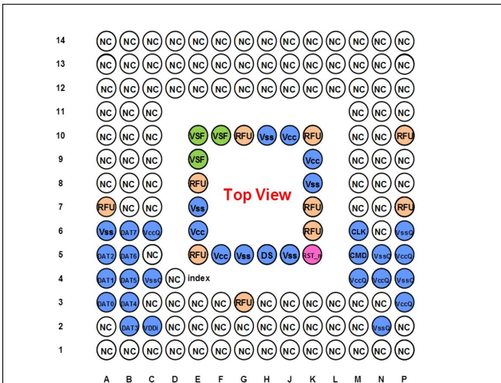
Figure 1 153 FBGA
