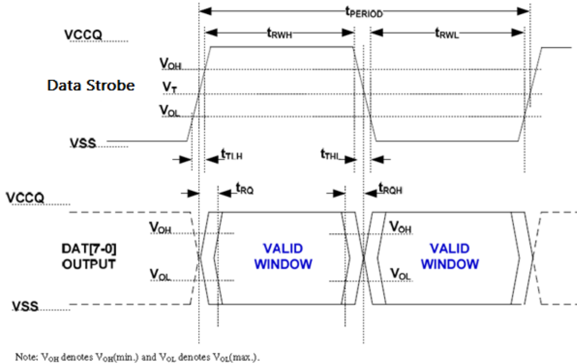
Figure 6 HS400 Device Output Timing
