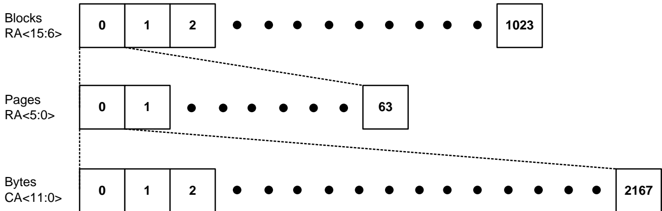
Figure 1-4. MKSV1GIW-BE
