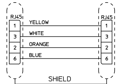
WIRING DIAGRAM
