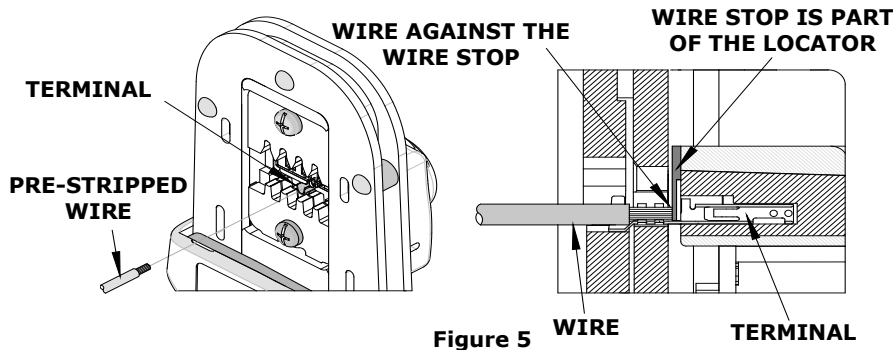
Figure 5 WIRE TERMINAL
