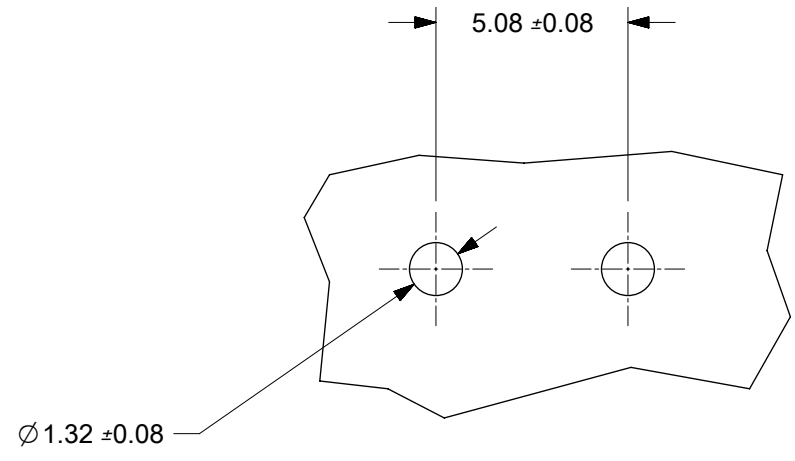
PRINTED CIRCUIT BOARD HOLE PATTERN
