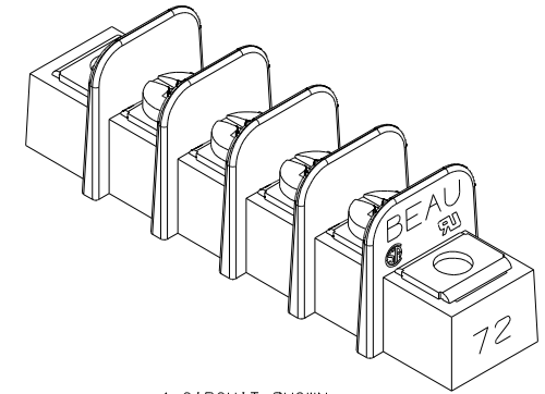
4 CIRCUIT SHOWN
