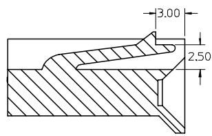
SECTION Z-Z
