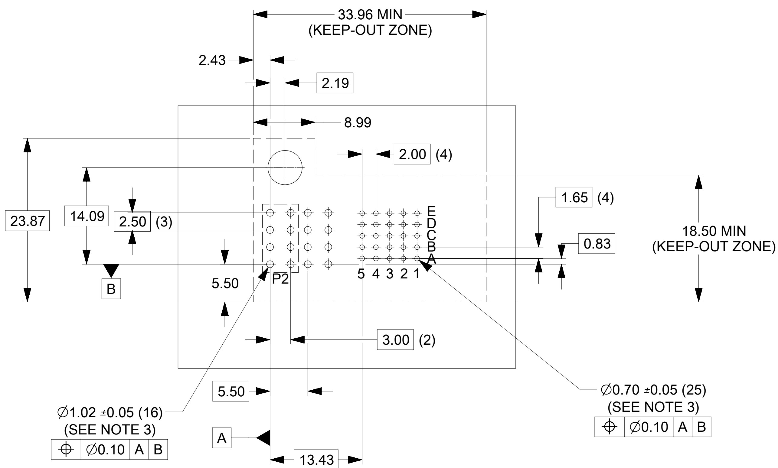
RECOMMENDED PCB LAYOUT AND KEEP-OUT ZONE
