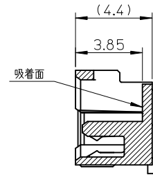
SECTION Y-Y
