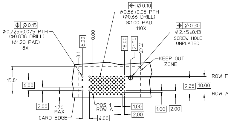
DAUGHTERCARD HOLE PATTERN (CONNECTOR SIDE)
