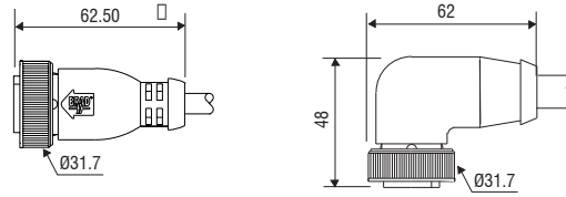
Mini-Change® Home Run Connectors for Micro-Change® Multi-Port
