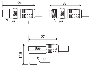
M23 Home Run Connectors for Micro-Change® Multi-Port
