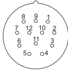
Female Connector Face View
