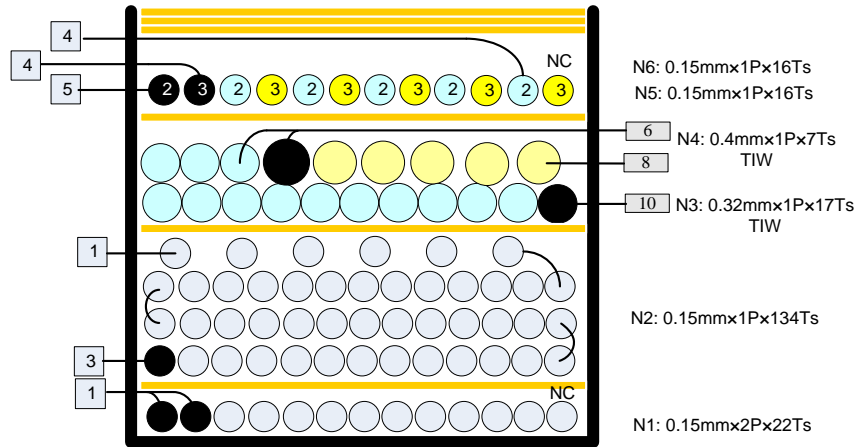
Figure 5—Winding Diagram
