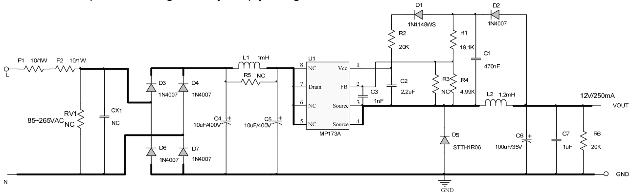
Figure 4: Reference schematic for 2kV surge
