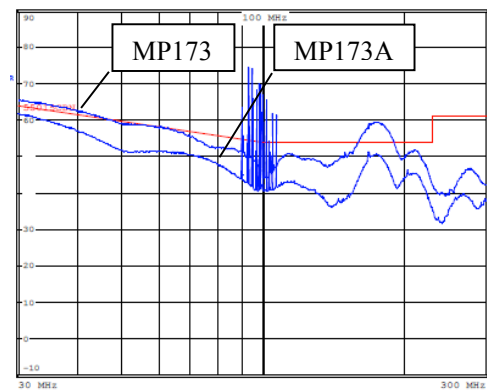
RE Performance
