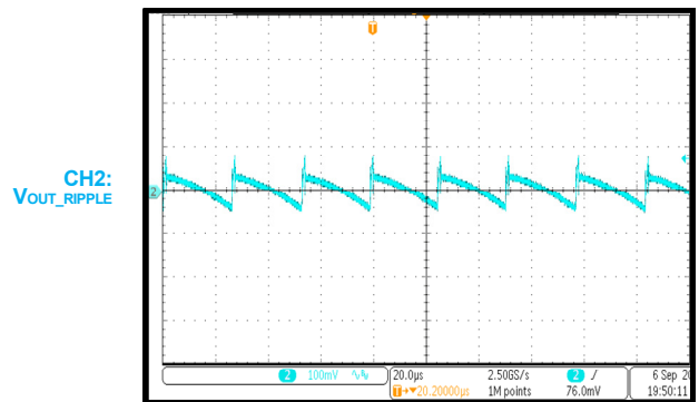
Output Ripple
