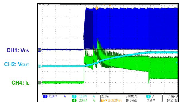
Start-Up
