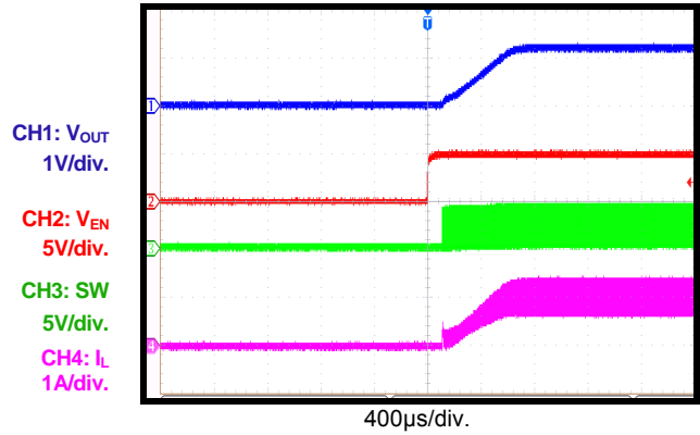
EN Power On V_{IN} = 5V , V_{OUT} = 1.2V , I_{OUT} = 1A
