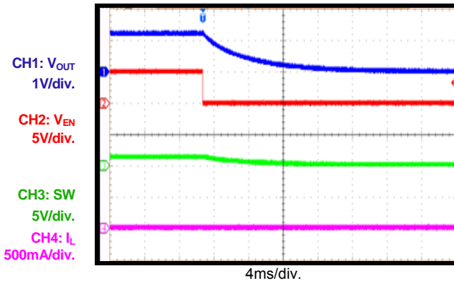
EN Power Off V_{IN} = 5V , V_{OUT} = 1.2V , I_{OUT} = 0A
