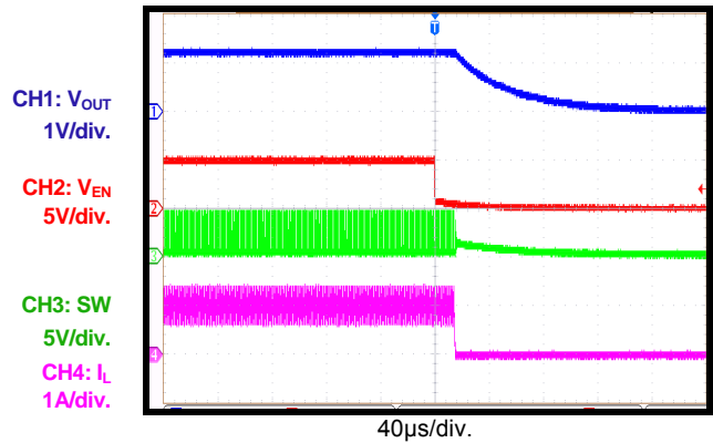
EN Power Off V_{IN} = 5V , V_{OUT} = 1.2V
