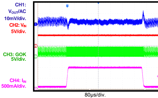
Load Transient V_{IN} = 5V , V_{OUT} = 1.2V , I_{OUT} = 0.1 \sim 1A
