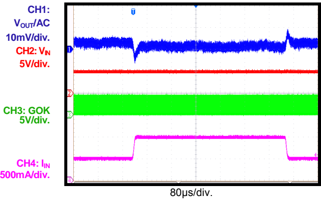
Load Transient V_{IN} = 5V , V_{OUT} = 1.2V
