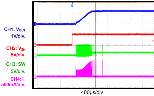
EN Power On V_{IN} = 5V , V_{OUT} = 1.2V , I_{OUT} = 0A
