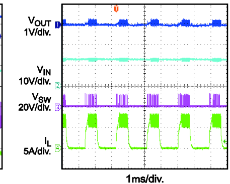
Short Circuit Steady I_{OUT}=3A
