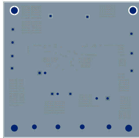
Figure 4—Mid 2 Layer
