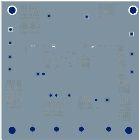
Figure 3—Mid 1 Layer
