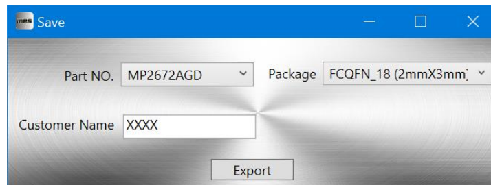
Figure 10: Exporting Configurations
