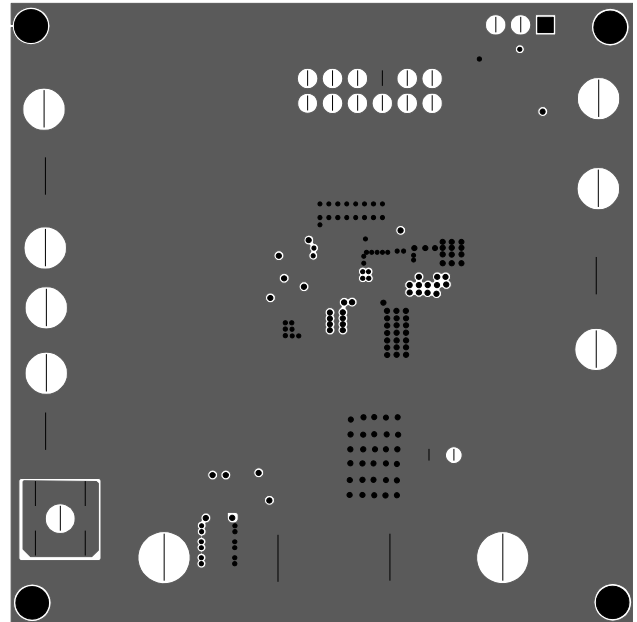
Figure 6-Inner3 Layer
