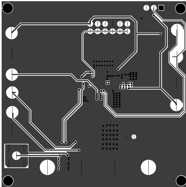
Figure 5-Inner2 Layer
