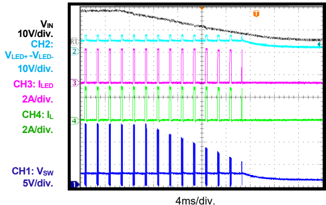
2-Step Dimming Shutdown through VIN
