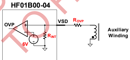
Figure 8—OVP Circuit
