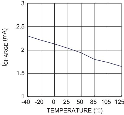
Charging Current From Pin D vs. Temperature (VCC=6V, Vdrain=400V)
