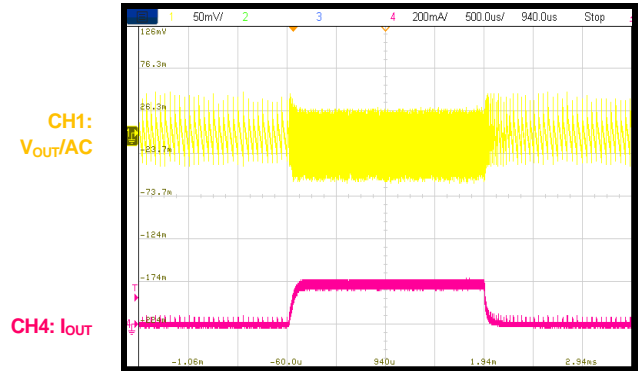
Load Transient
