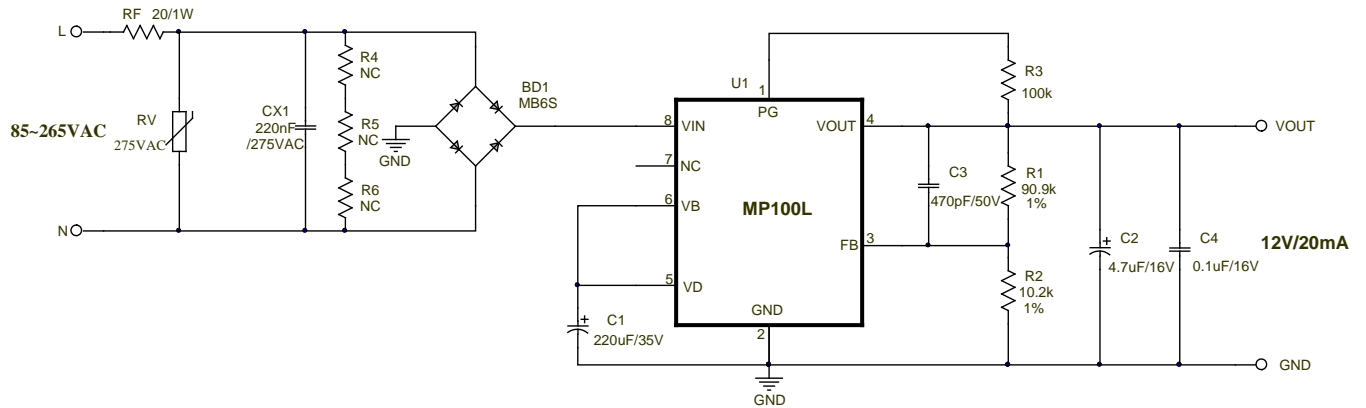
Figure 4: Typical Application
