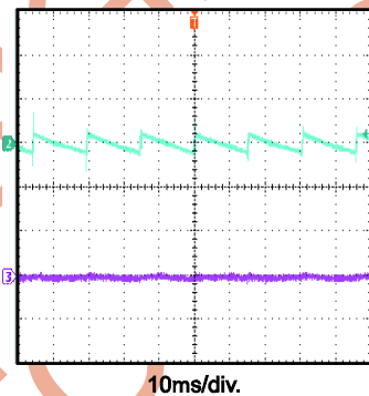
Output Ripple 230Vac, No Load
