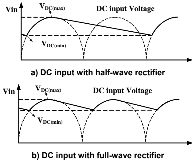
Figure 7: Input voltage waveform
