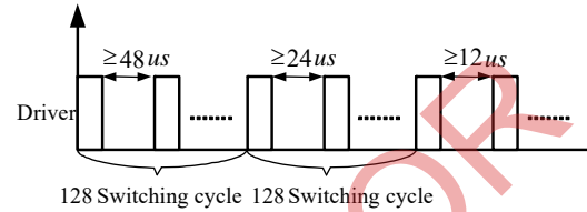
Figure 2— t_{\text{minoff}} at start-up Constant Voltage (CV) Operation
