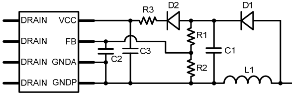
Figure 6: External Feedback Circuit with Dedicated Feedback Circuit
