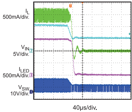
V_{IN} Shutdown
