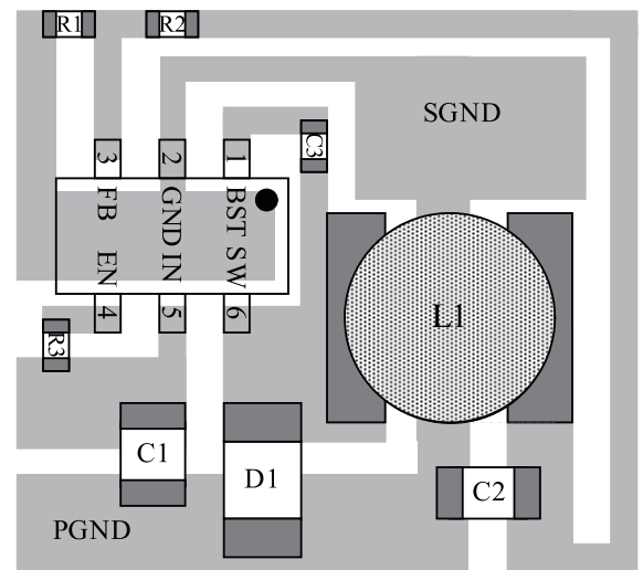
Figure 2: PCB Layout
