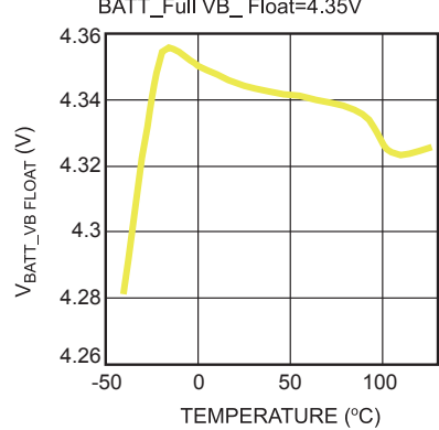
BATT_Full VB Float vs. Temperature
