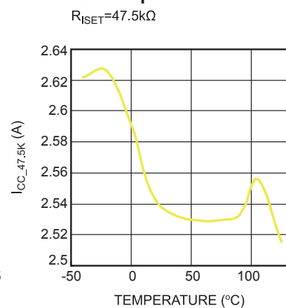
CC Charge Current vs. Temperature
