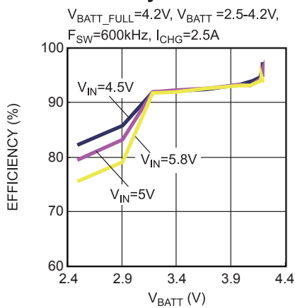
Constant Current Charge Efficiency
