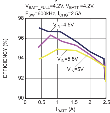
Constant Voltage Charge Efficiency
