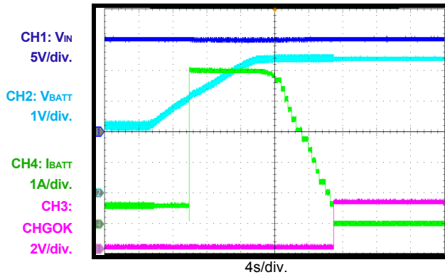
Battery Charge Curve V_{IN} = 15V , R_{LIM} = 71.5k\Omega , R_{SET} = 42.2k\Omega
