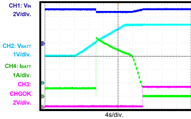
Battery Charge Curve V_{IN} = 5V , R_{LIM} = 71.5k\Omega , R_{SET} = 42.2k\Omega
