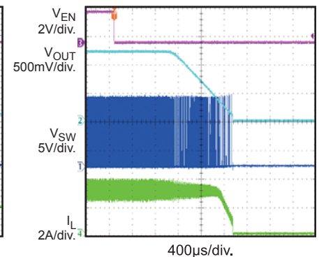
Power down through EN I_{OUT} = 3A(CC-Load)
