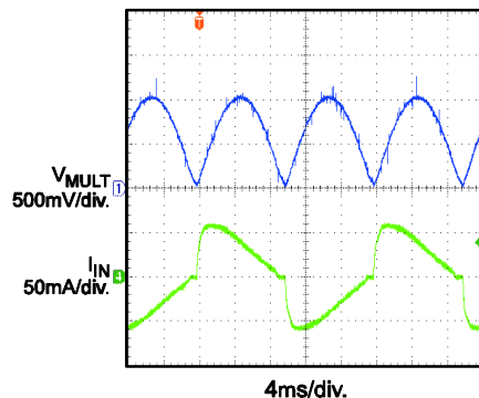
Input Voltage and Current V_{IN}=230V_{AC}/50\text{Hz} , Full Load
