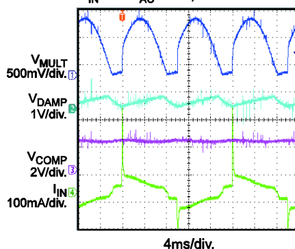
Dimming Performance Max dimming on phase with leading-edge dimmer V_{IN}=230V_{AC}/50\text{Hz} , with dimmer
