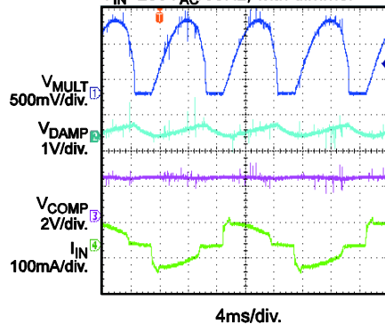
Dimming Performance Max dimming on phase with trailing-edge dimmer V_{IN}=230V_{AC}/50\text{Hz} , with dimmer
