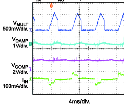
Dimming Performance Min dimming on phase with trailing-edge dimmer V_{IN}=230V_{AC}/50\text{Hz} , with dimmer
