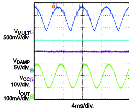
Steady State V_{IN}=230V_{AC}/50\text{Hz} , Full Load
