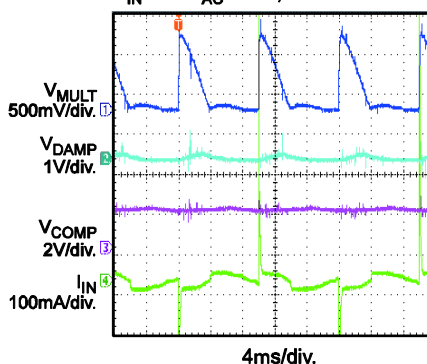
Dimming Performance Min dimming on phase with leading-edge dimmer V_{IN}=230V_{AC}/50\text{Hz} , with dimmer
