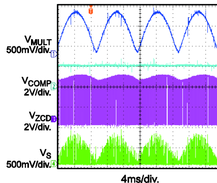
Steady State V_{IN}=230V_{AC}/50\text{Hz} , Full Load
