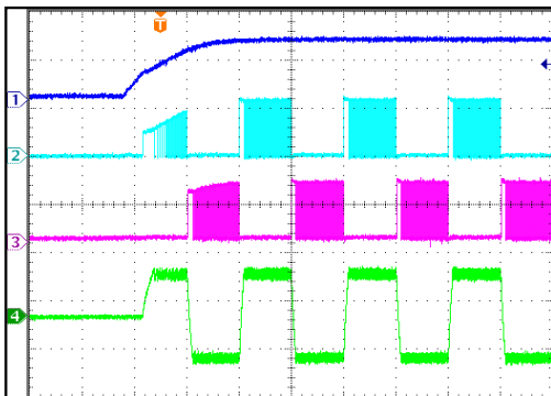
Power Ramp-Up, Full-Step
