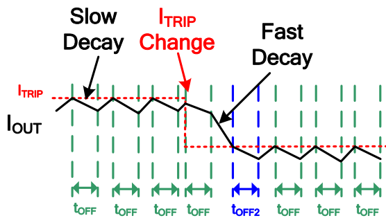
Figure 4: Slow Decay During t_{OFF} unless I_{OUT} > I_{TRIP} at end of t_{OFF}
