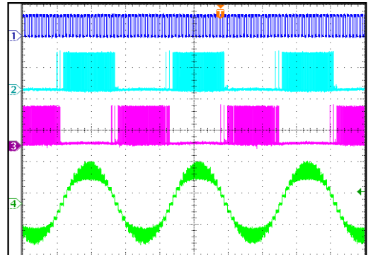
Steady State, Eighth-Step
