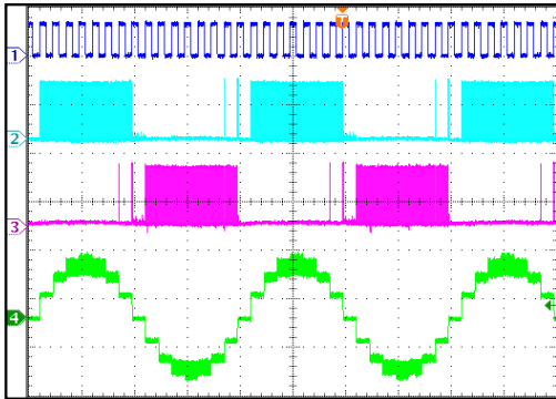
Steady State, Quarter-Step
