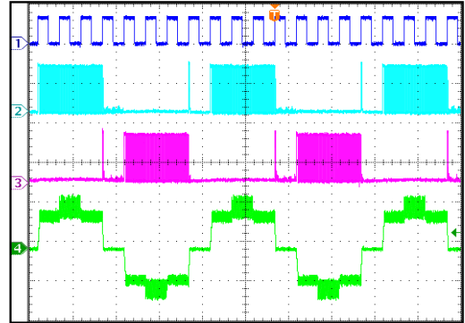
Steady State, Half-Step
