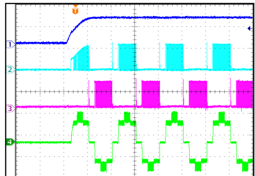
Power Ramp-Up, Half-Step
