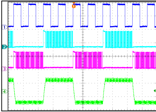
Steady State, Full-Step
