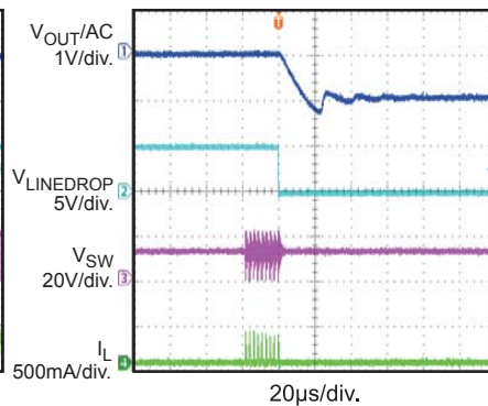
19V to 18V Switching I_{OUT} = 0A
