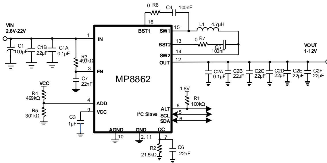
Figure 14: Typical Application Circuit for 1V-12V out
