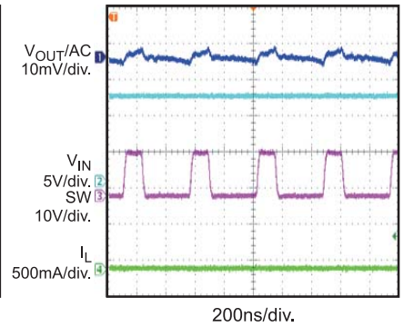
Output Ripple
