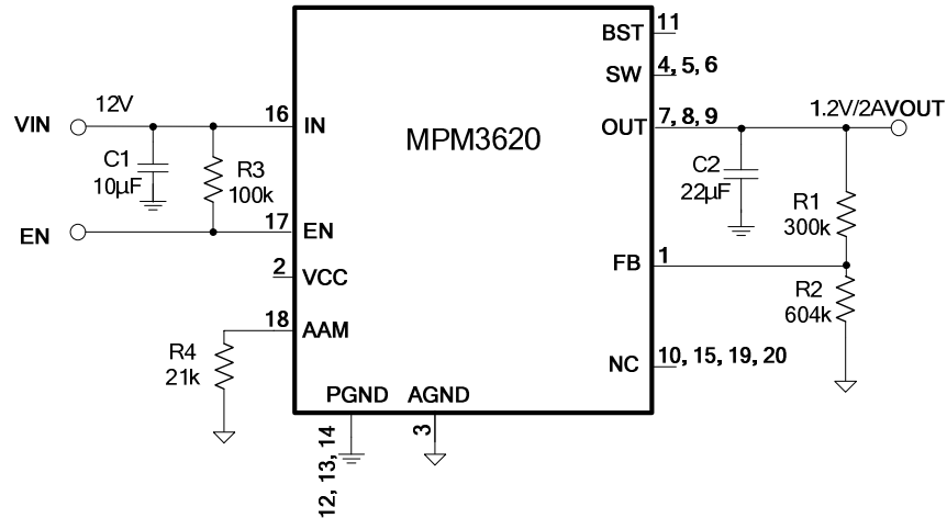
Figure 17. V_{OUT}=1.2V , I_{OUT}=2A
