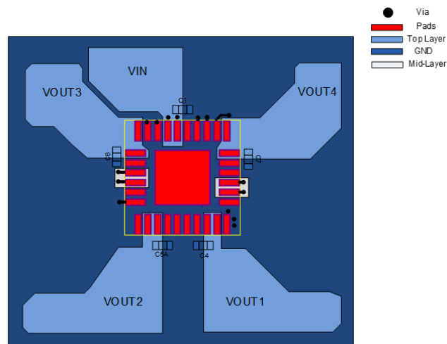
Figure 15: Recommended PCB Layout
