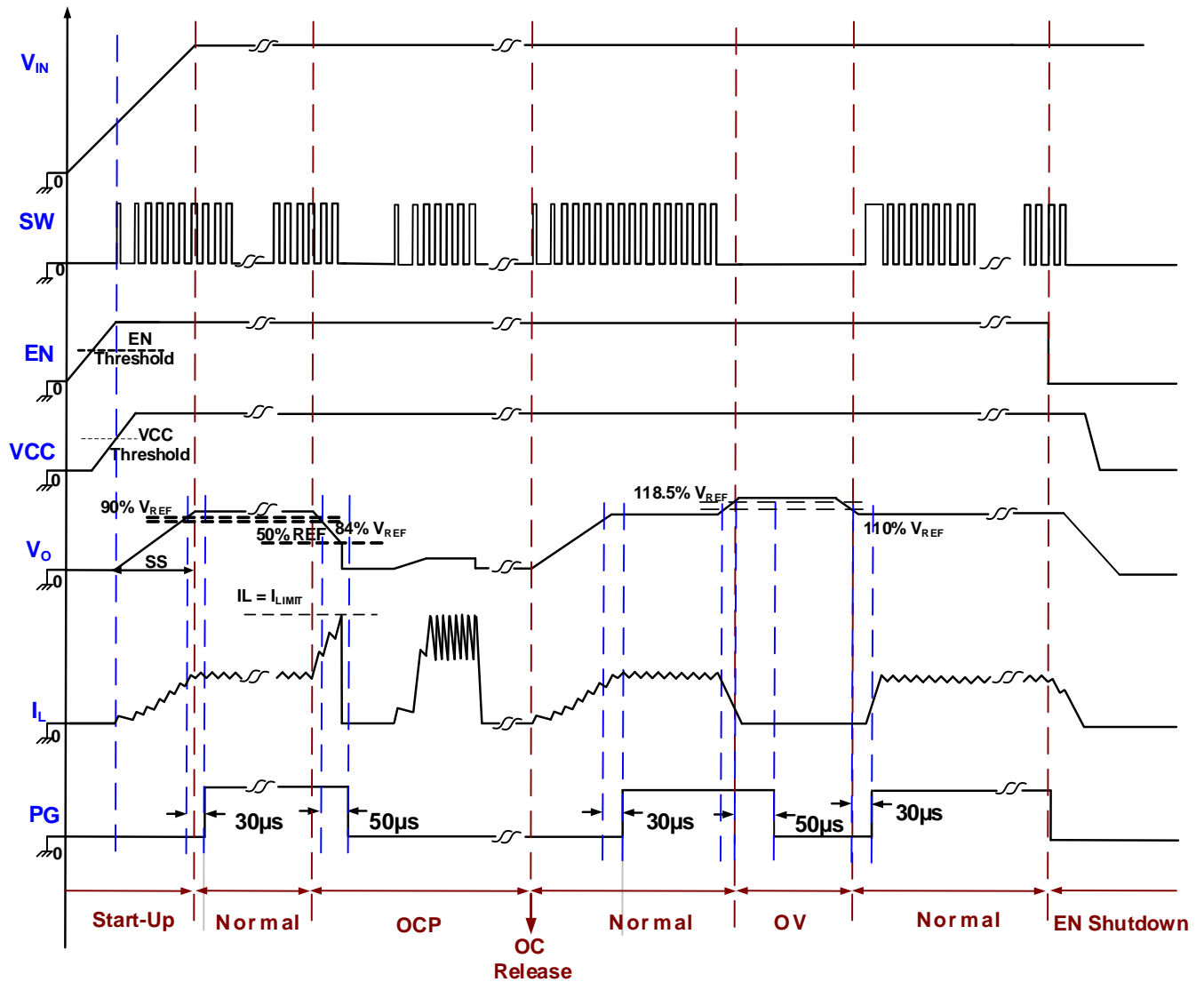
Figure 2: Timing Sequence
