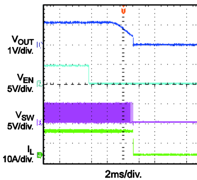
Shutdown Through EN I_{OUT} = 12A
