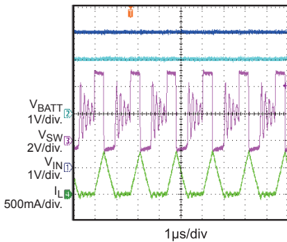
TC Charge Steady State V_{BATT\_FULL}=4.2V , V_{BATT}=2V , F_{SW}=600kHz
