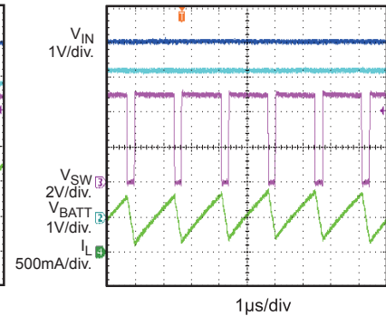
CV Charge Steady State V_{BATT\_FULL}=4.2V , V_{BATT}=4.2V , F_{SW}=600kHz
