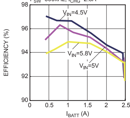
Constant Voltage Charge Efficiency
