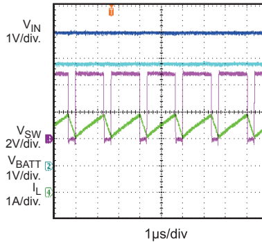
CC Charge Steady State V_{BATT\_FULL}=4.2V , V_{BATT}=3.7V , F_{SW}=600kHz
