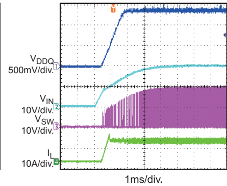
Start-Up through V_IN I_{OUT} = 10A
