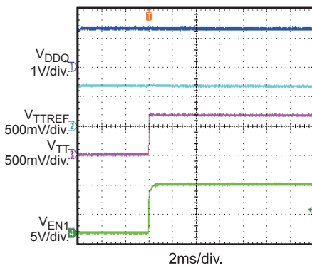
V TT Start-Up through EN1 I_{OUT} = 0A
