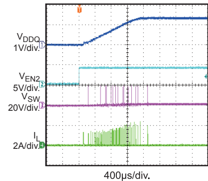
Start-Up through EN I_{OUT} = 0A
