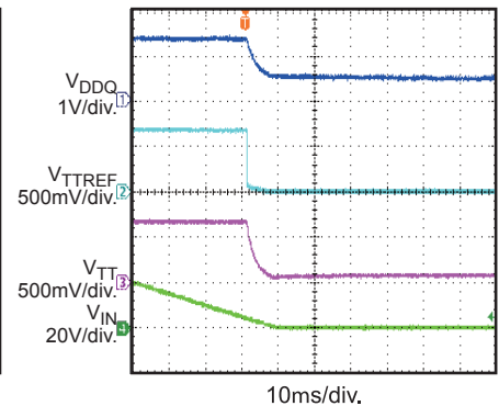
V TT &V TTREF Shutdown through V IN I_{OUT} = 0A
