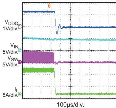
Shutdown through V_IN I_{OUT} = 10A
