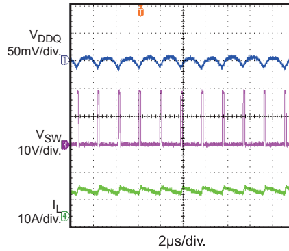
Output Voltage Ripple I_{OUT} = 10A
