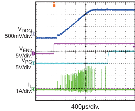
Power Good through EN Start-Up I_{OUT} = 0A
