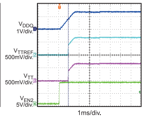
V TT &V TTREF Start-Up through EN2 I_{OUT} = 0A
