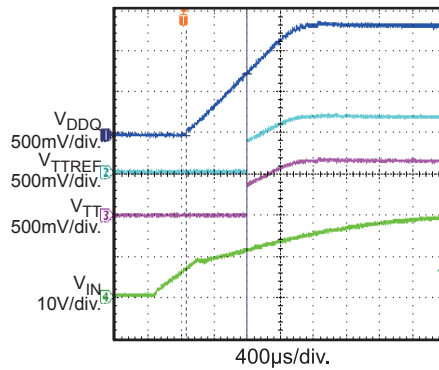
V TT &V TTREF Start-Up through V IN I_{OUT} = 0A
