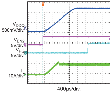
Power Good through EN Start-Up I_{OUT} = 10A
