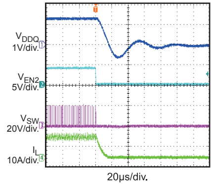
Shutdown through EN I_{OUT} = 10A
