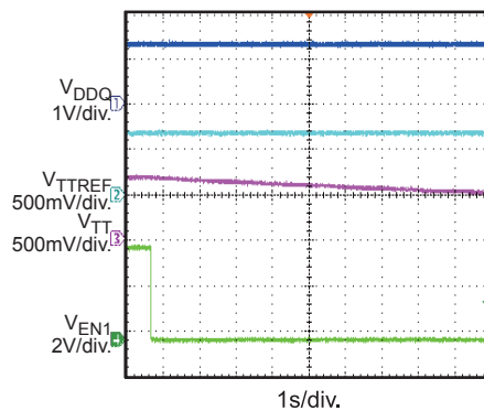
V TT Shutdown through EN1 I_{OUT} = 0A
