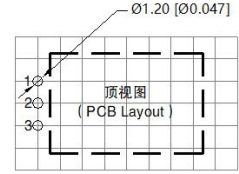
K78xx-2000R3L
