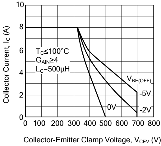
Figure 8. Maximum Reverse Bias Switching Safe Operating Area
