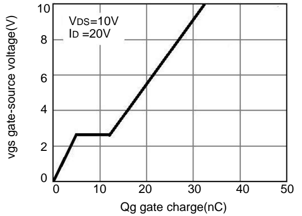
Fig.4 gate charge
