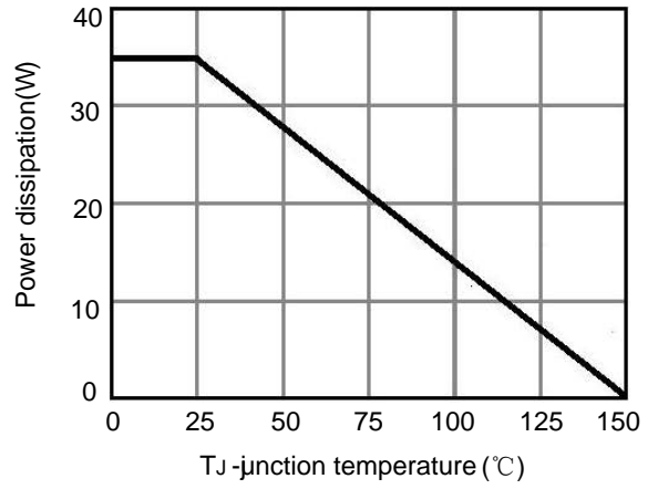
Fig.8 power de-rating
