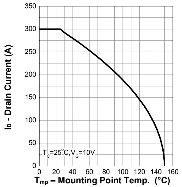
Current Capability
