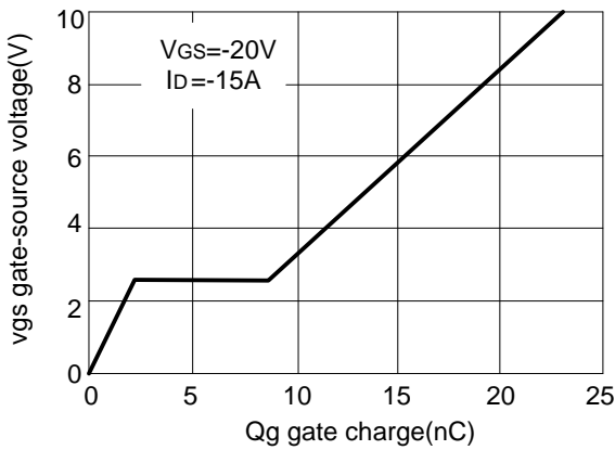
Fig.9 gate charge
