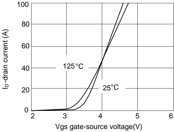
Figure 3 Transfer characteristics
